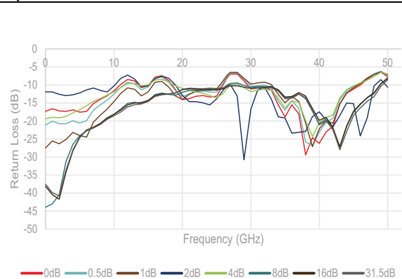
Figure 12 ■ Input Return Loss (Major Attenuation States)
