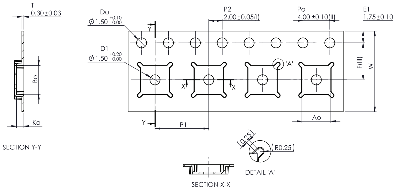
Figure 40 ■ Tape and Reel Specifications for 24-lead 4 x 4 mm LGA
