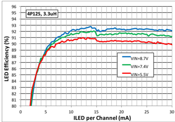
Figure 38. 2S, 4P12S LED Efficiency, 3.3 \mu\text{H} Inductor
