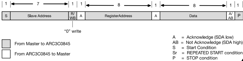
Figure 59. "Write" Data Transfer Format in Standard, Fast, Fast-Plus Modes
