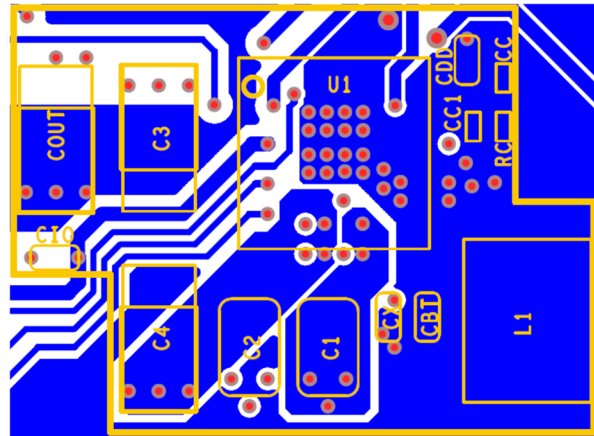
Figure 66. Bottom Layer
