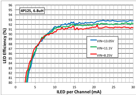
Figure 24. 4P12S LED Efficiency, 6.8 \mu\text{H} Inductor
