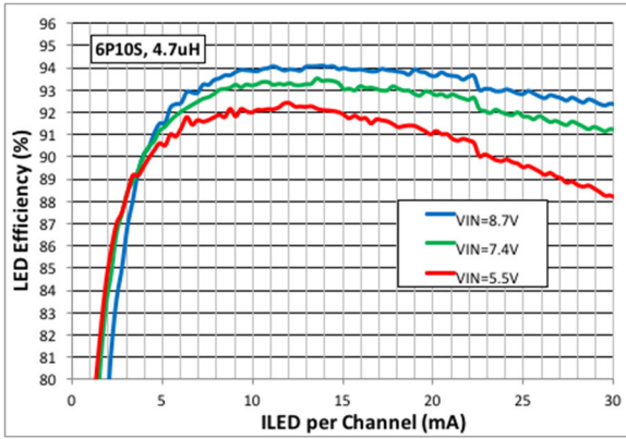
Figure 14. 6P10S LED Efficiency, 4.7 \mu\text{H} Inductor
