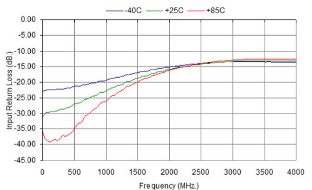
Figure 7 • Input Return Loss vs Temperature @ 12 dB State
