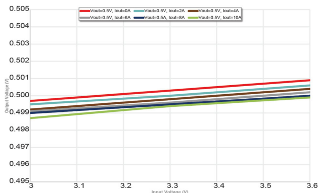
Figure 7. Line Step Output Voltage vs. Input Voltage Single-Device, V_{OUT} = 0.5V (Line Regulation, mV/V )
