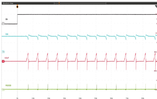
Figure 15. Startup into Short Circuit
