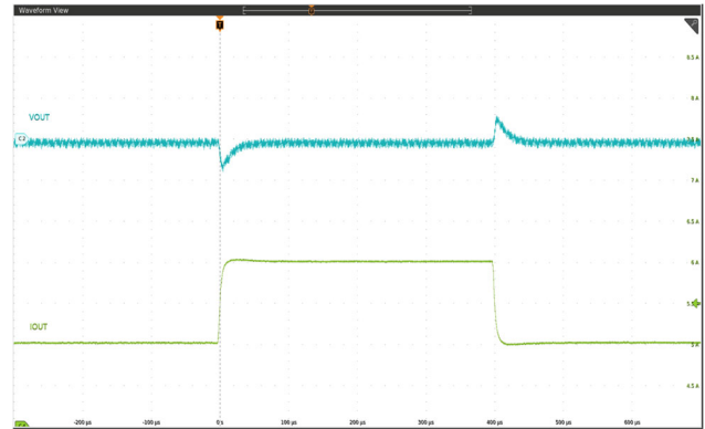
Figure 12. Load Transient 5A to 6A, 0.2A/\mu s , V_{IN} = 3.3V , V_{OUT} = 0.5V
