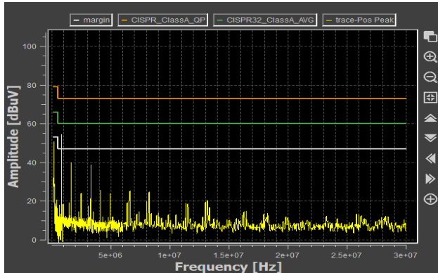
Figure 17. Conducted EMI ( V_{OUT} ) Single EVK, V_{IN} = 3.3V , V_{OUT} = 0.5V , I_{OUT} = 6A
