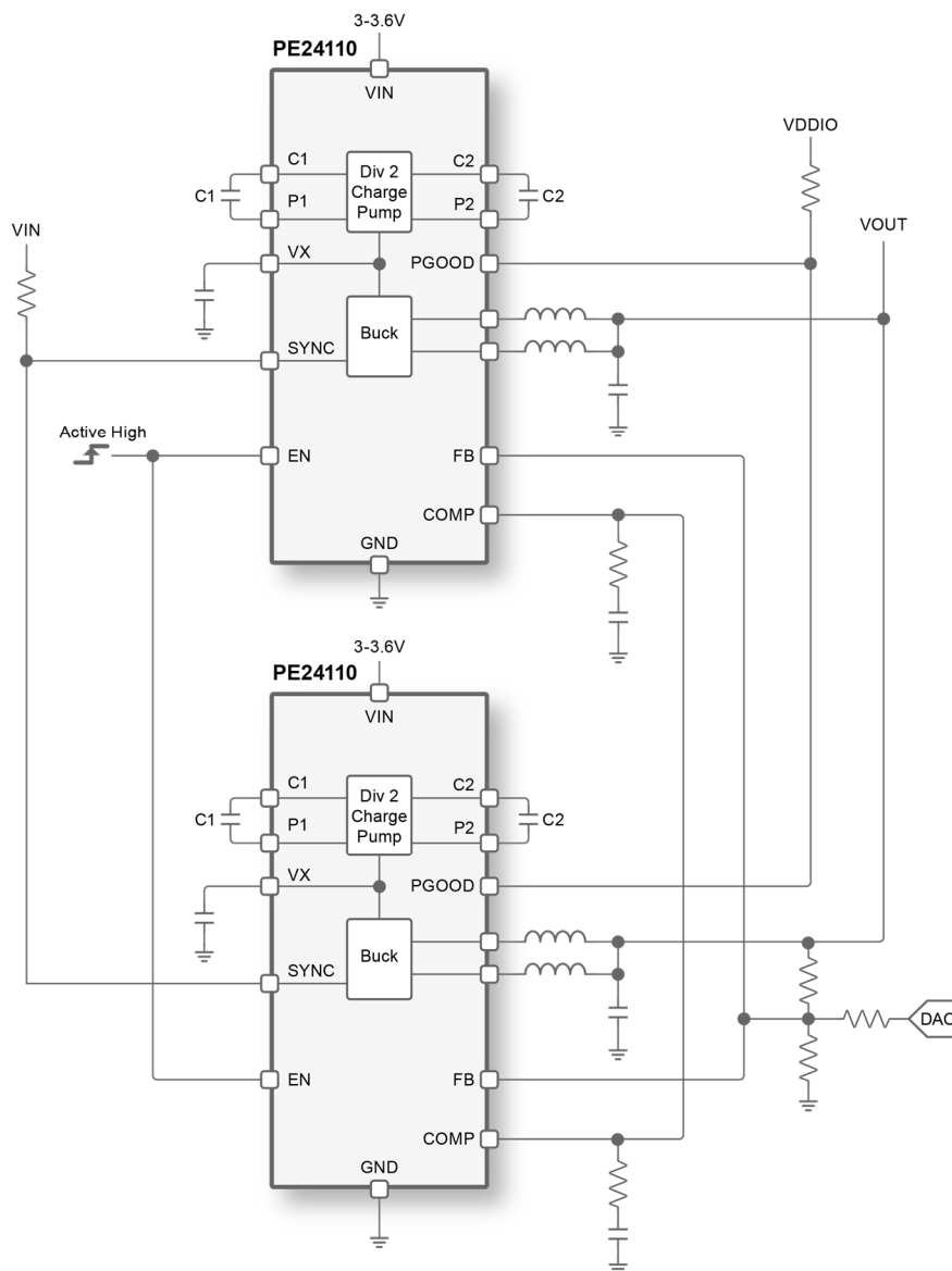
Figure 24. Using Two PE24110 Parts in Parallel
