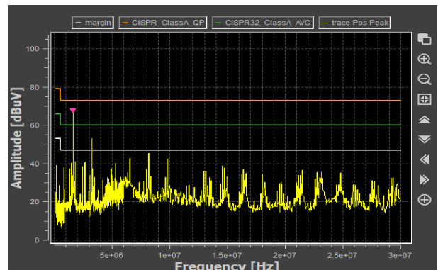
Figure 16. Conducted EMI (Input) Single EVK, V_{IN} = 3.3V , V_{OUT} = 0.5V , I_{OUT} = 6A
