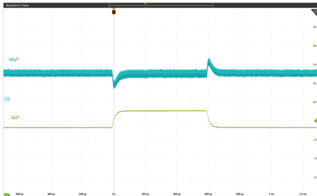
Figure 13. Load Transient 20% 7.2A-9A, 0.5A/\mu s , V_{IN} = 3.3V , V_{OUT} = 0.5V
