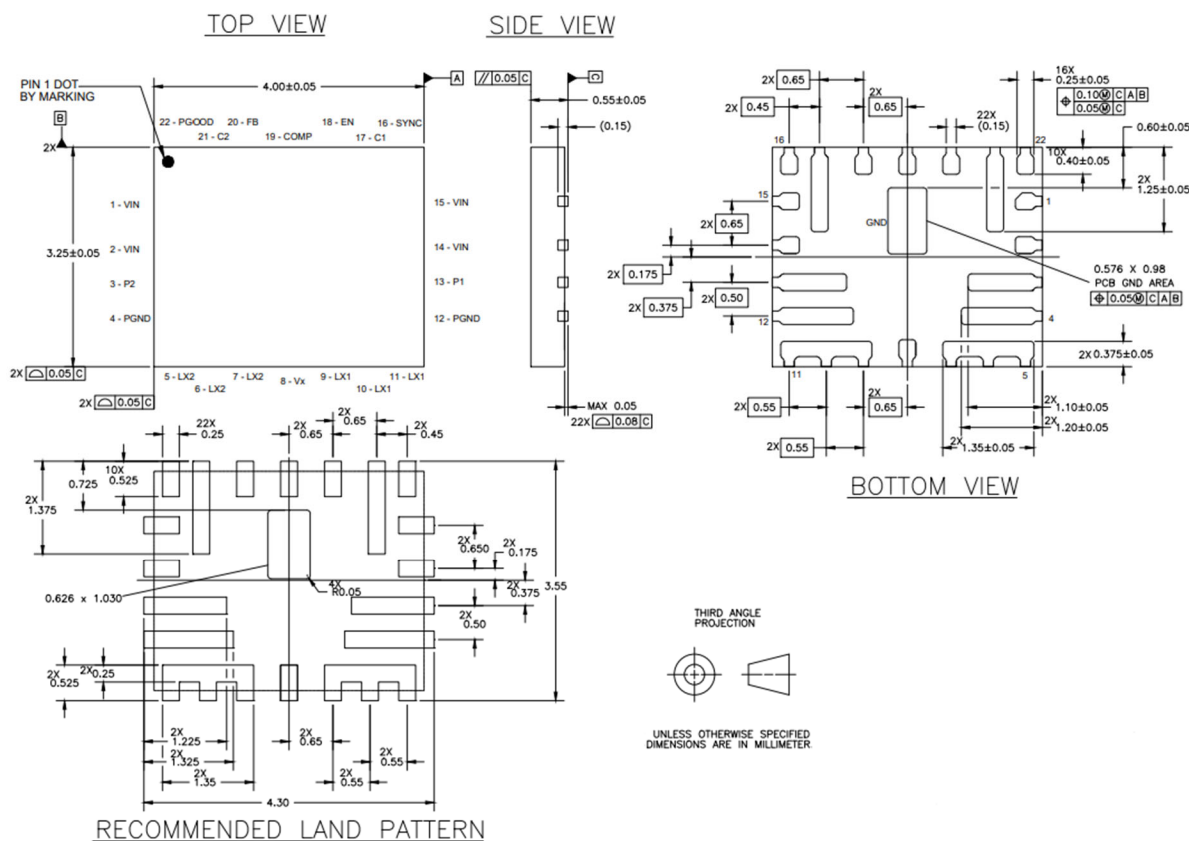
Figure 30. Package Drawing QFN 4 mm x 3.25 mm x 0.55 mm
