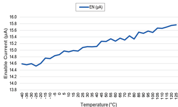
Figure 9. EN Pin Leakage vs. Temperature
