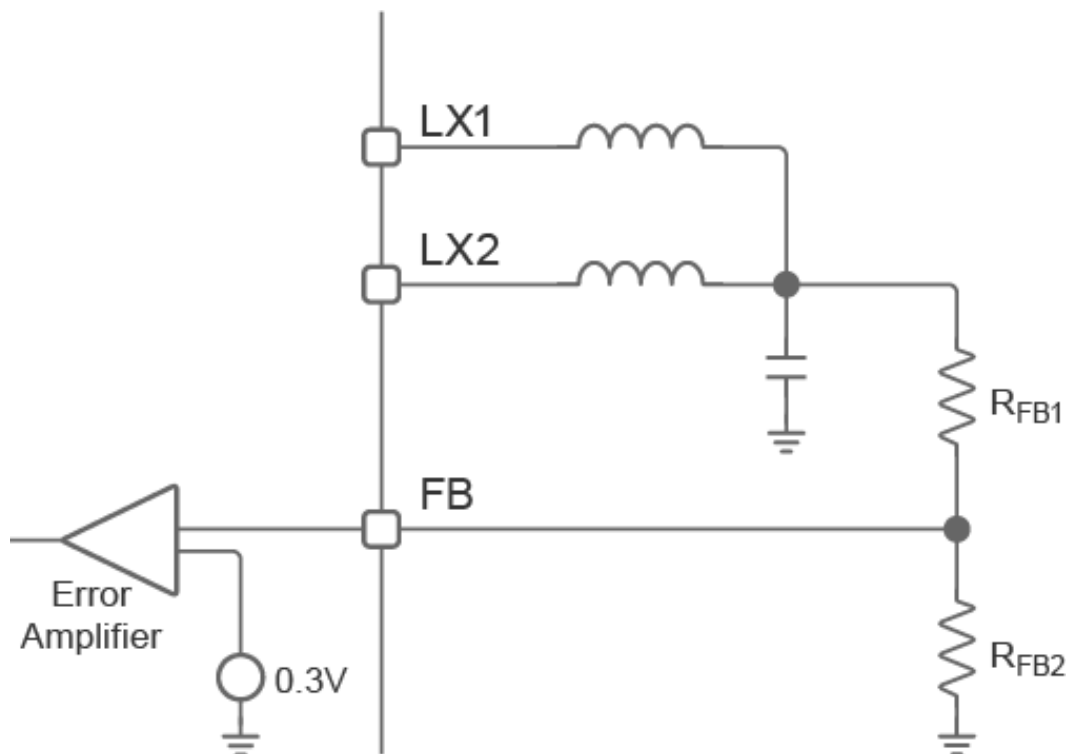
Figure 22. Setting the Output Voltage with External Feedback Resistors
