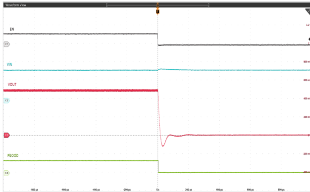
Figure 11. Shutdown into Load V_{IN} = 3.3V , V_{OUT} = 0.5V , I_{OUT} = 6A
