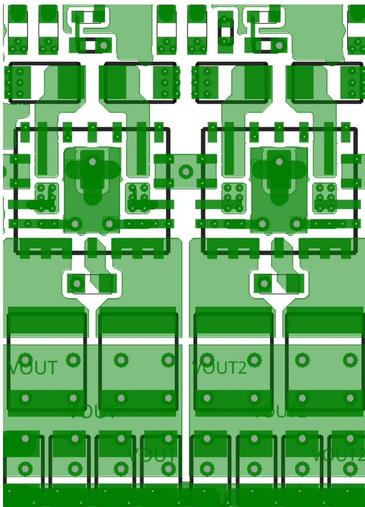
Figure 25. Example Layout of Two Parallel Devices
