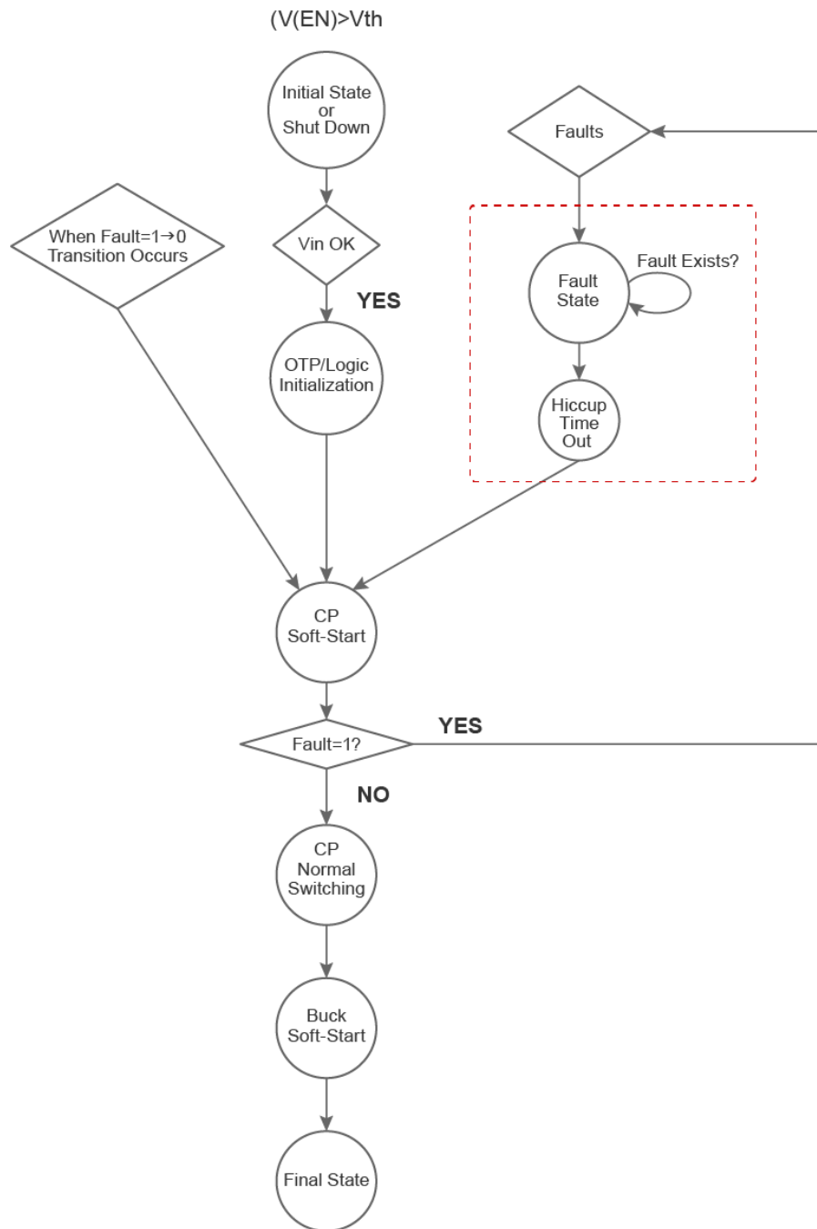
Figure 23. Power-up Sequence
