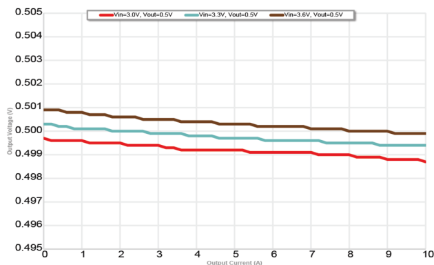
Figure 6. Output Voltage vs. Output Current Single-Device, V_{OUT} = 0.5V
