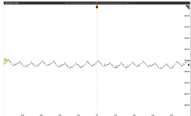
Figure 14. Output Ripple Single EVK, V_{IN} = 3.3V , V_{OUT} = 0.5V , I = 9A
