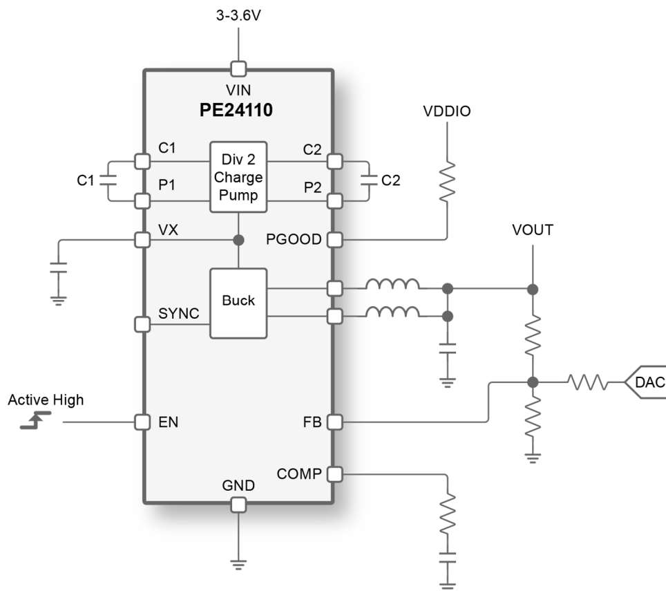
Figure 27. Adjusting the Output Voltage with External DAC
