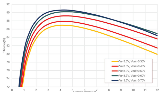
Figure 5. Efficiency vs. Load Current V_{IN} = 3.3V , V_{OUT} = 0.35V, 0.4V, 0.5V, 0.6V, 0.7V Single-Device F_{sw} = 800\text{ kHz}
