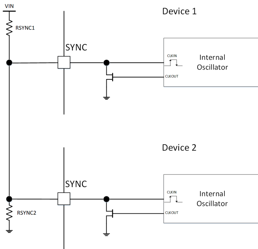
Figure 26. Sync Connections for Parallel Operation
