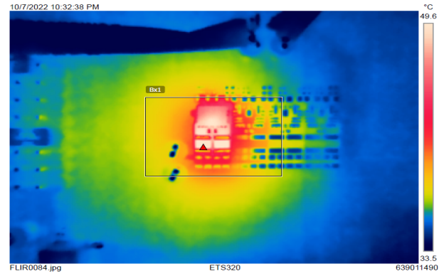
Figure 18. Thermal Plot Single Device, V_{IN} = 3.3V , V_{OUT} = 0.5V , I_{OUT} = 10A
