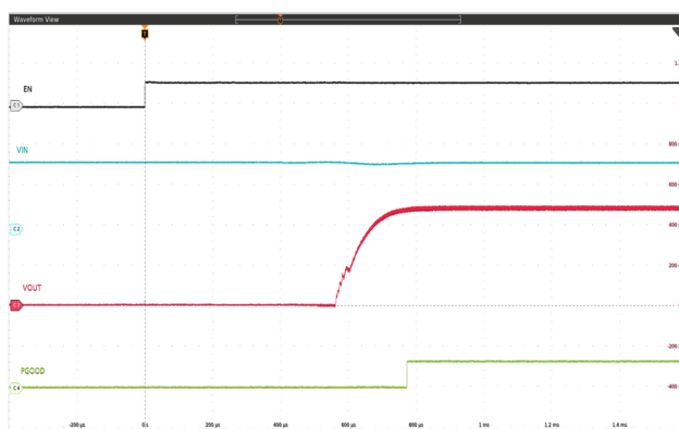
Figure 10. Startup into Load V_{IN} = 3.3V , V_{OUT} = 0.5V , I_{OUT} = 6A
